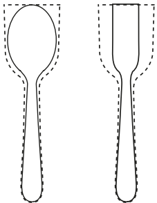
3 Rifilatura Overall cutting on outside blank
